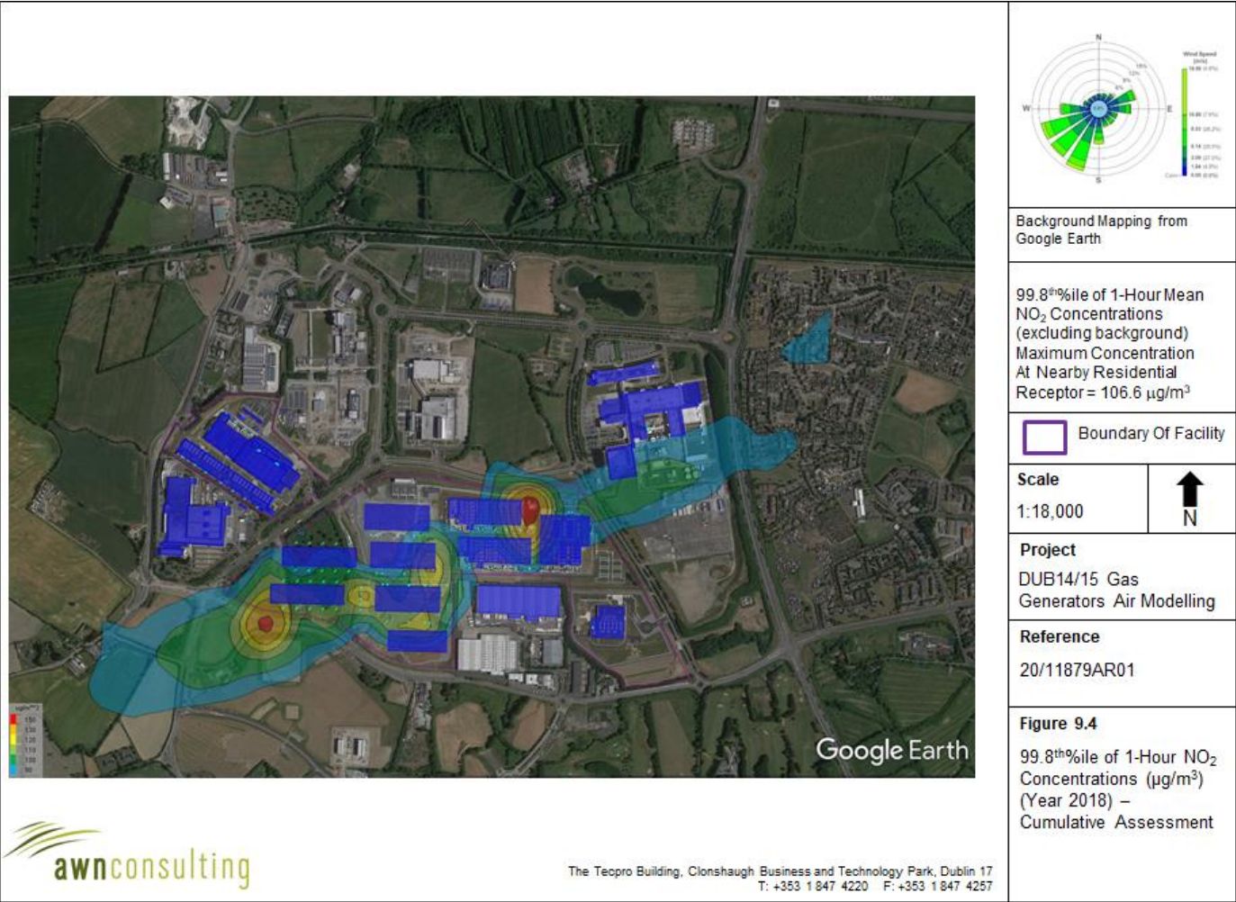
Figure 9.4: Cumulative Operations – 99.8 th %ile of 1-Hour NO 2 Concentrations (µg/m 3 ) (Year 2018)
