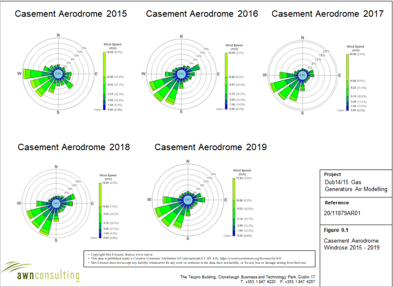
Figure 9.1: Casement Aerodrome Windrose (2015 – 2019)
