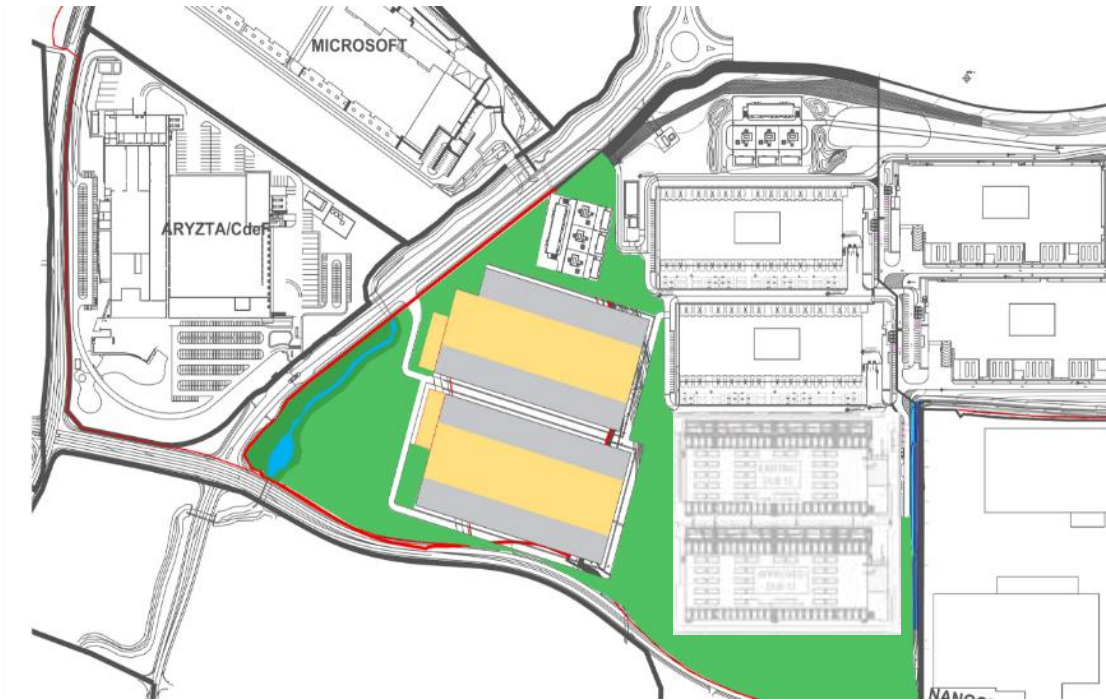
Figure 2.2 Double storey data centres option
