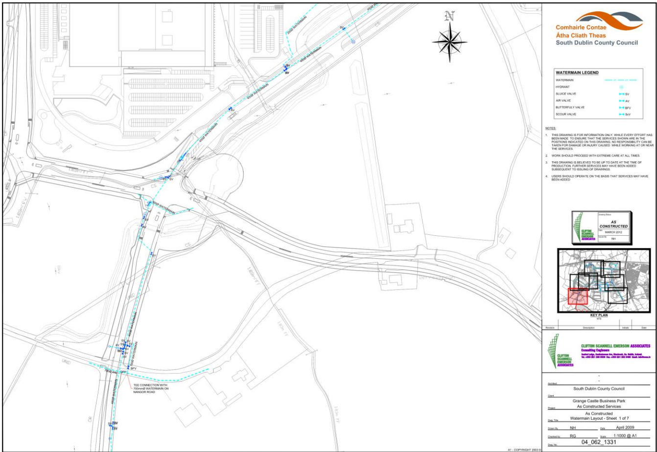
Figure 7.3 Irish Water / South Dublin County Council Water Infrastructure.
