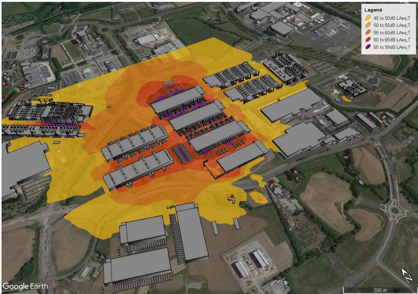
Figure 8.7: Scenario B – Day to Day (with DUB 14 and 15) with Gas Generation Contour (Extent of 45dB(A) Contour)
