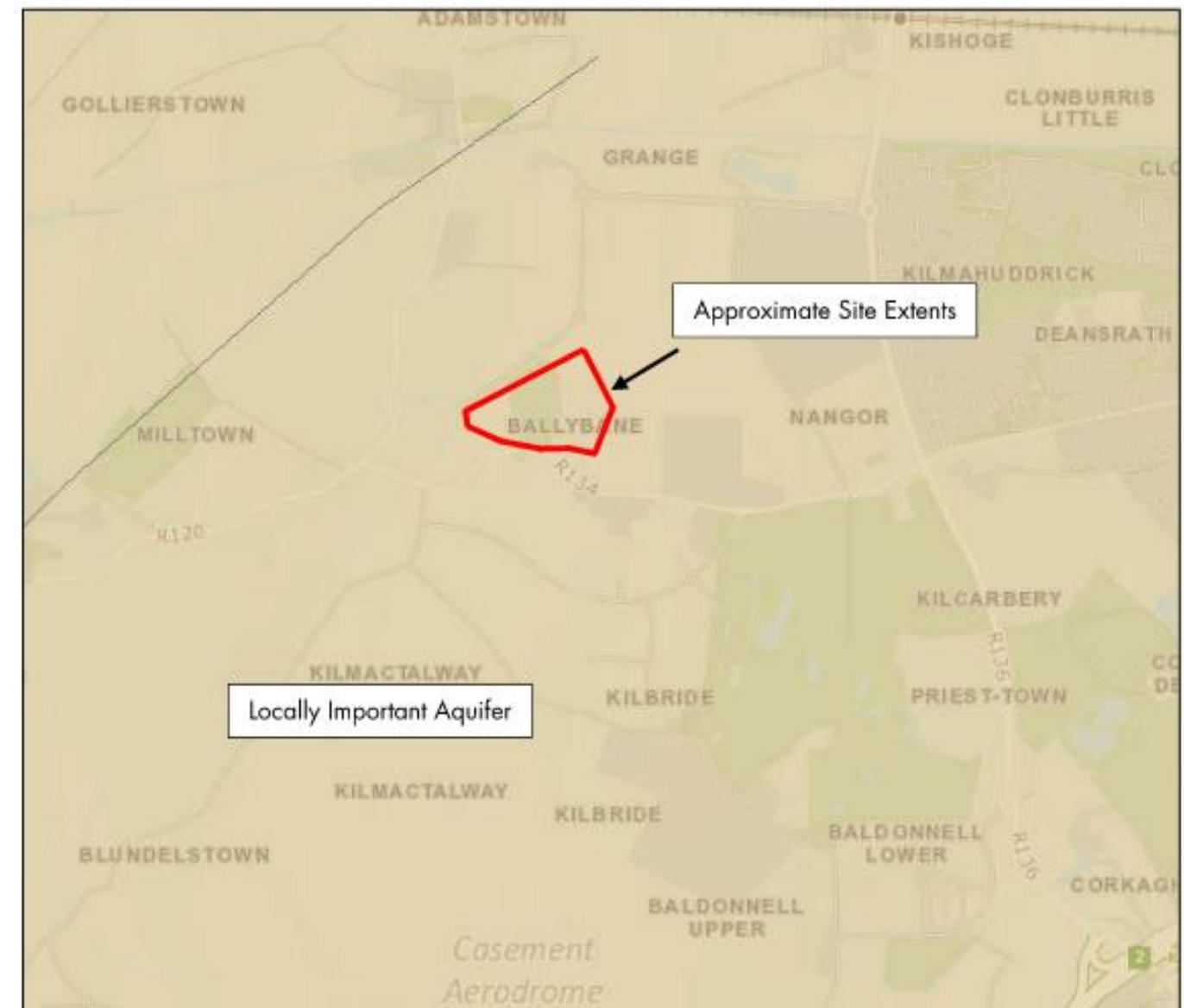
Figure 7.5. Bedrock Aquifer Classification (GSI online)
