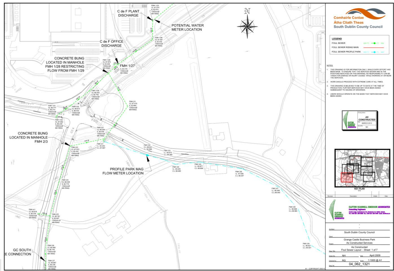
Figure 7.2 Irish Water / South Dublin County Council Foul Sewer Infrastructure.
