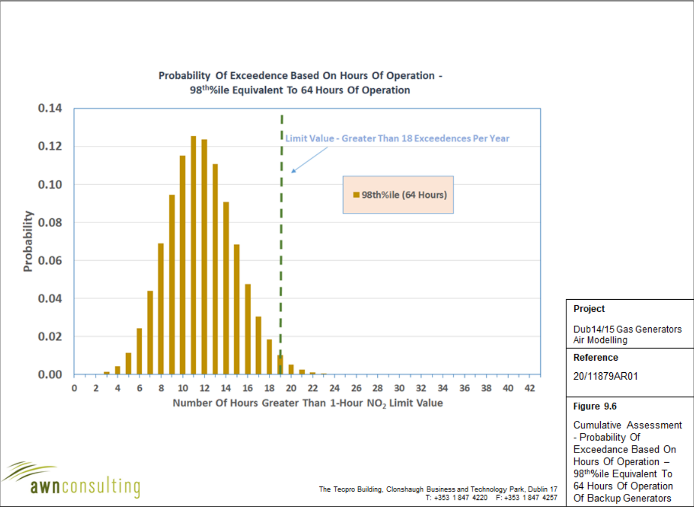
Figure 9.6: Cumulative Assessment – Probability of Exceedance Based On Hours Of Operation
