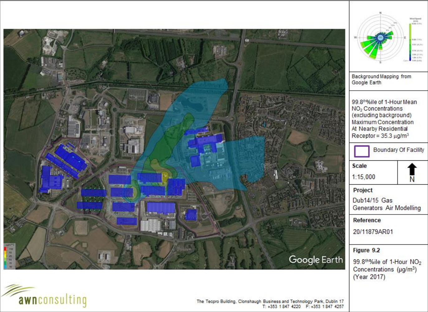
Figure 9.2: Gas Generators – 99.8 th %ile of 1-Hour NO 2 Concentrations (µg/m 3 ) (Year 2017)
