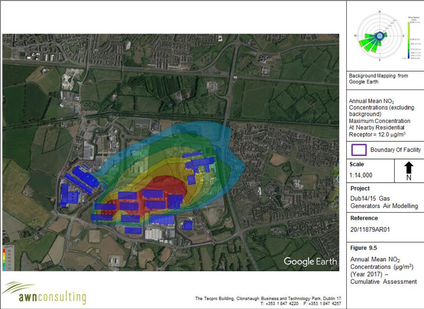
Figure 9.5: Gas Generators – Annual Mean NO 2 Concentrations (µg/m 3 ) (Year 2017)
