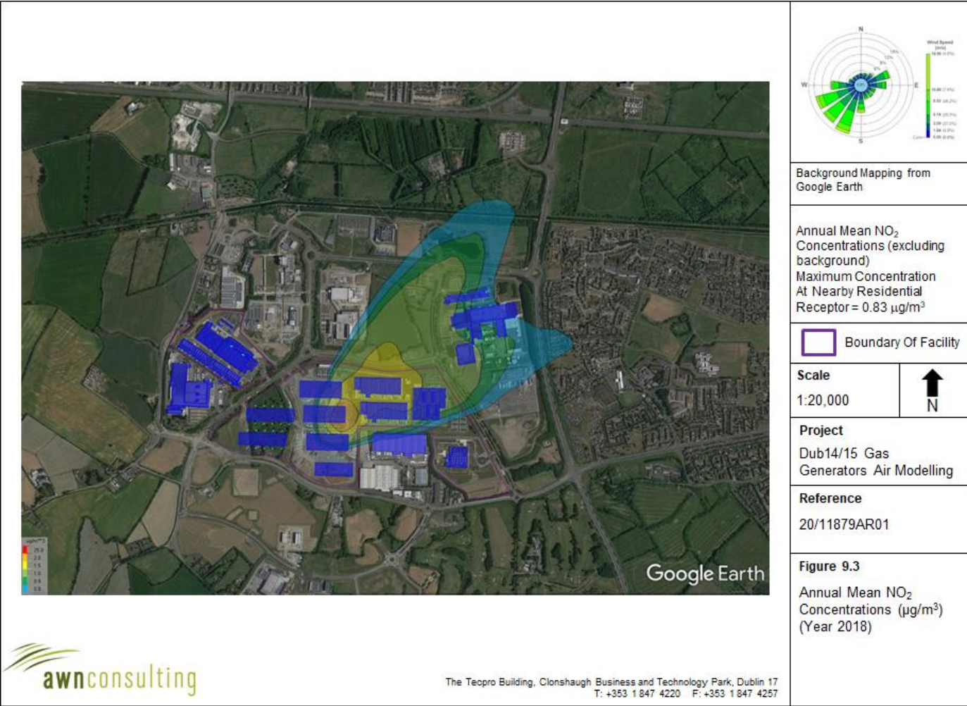
Figure 9.3: Gas Generators – Annual Mean NO 2 Concentrations (µg/m 3 ) (Year 2017)
