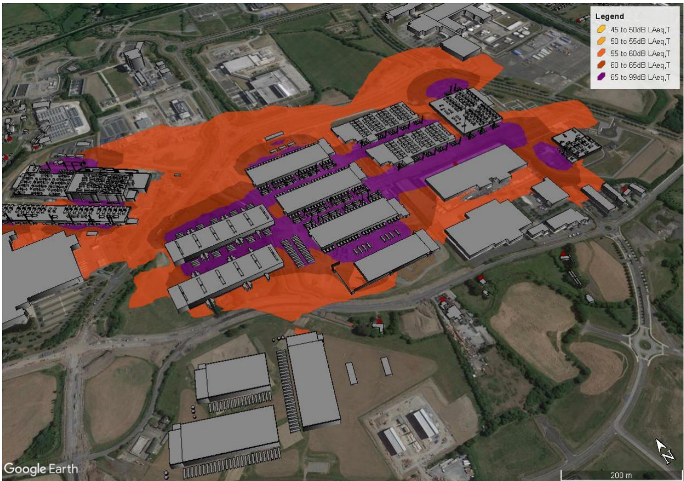
Figure 8.8: Scenario C – Emergency Operations (with DUB 14 and 15) Contour (Extent of 55dB(A) Contour)
