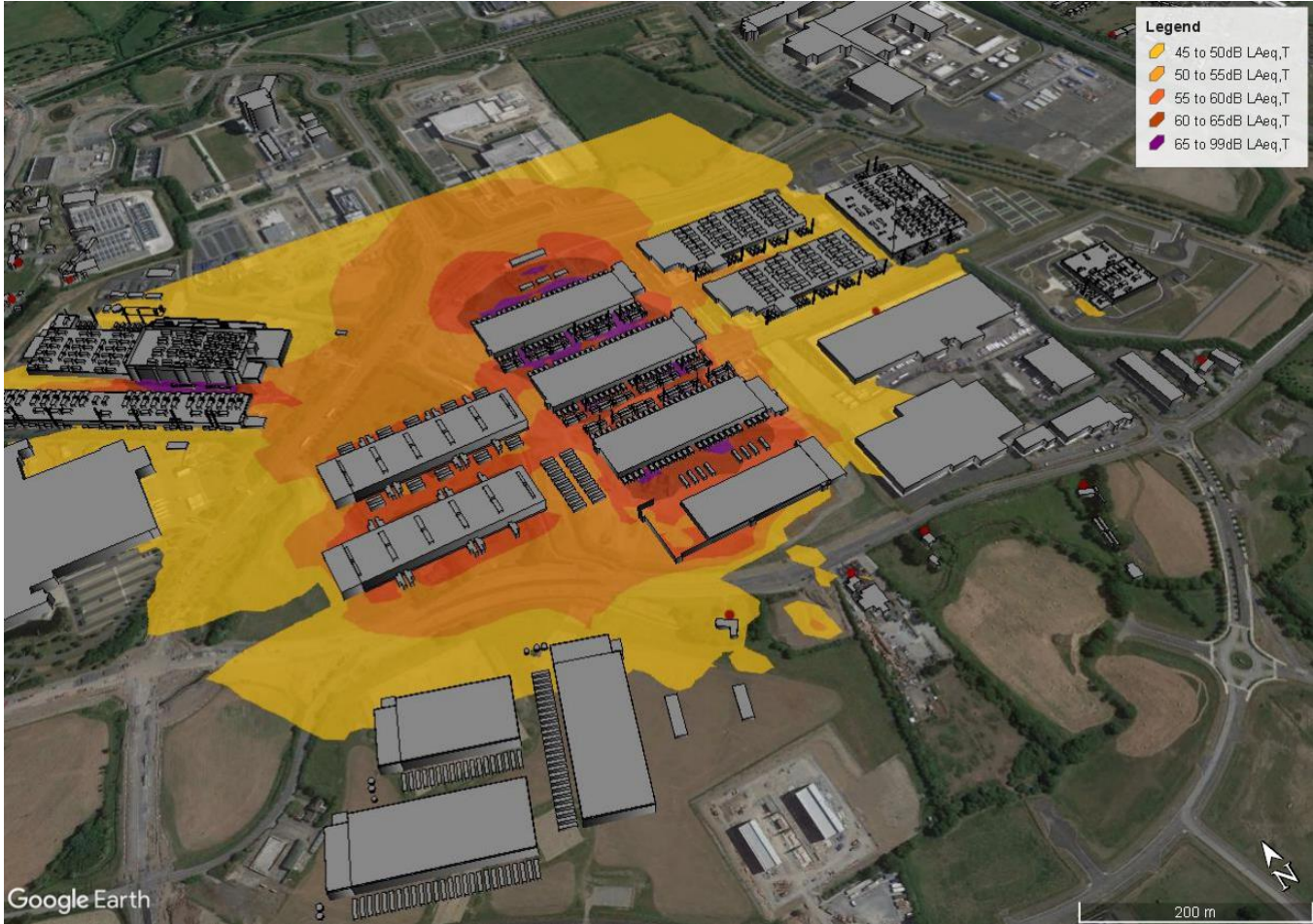
Figure 8.6: Scenario A – Day to Day (with DUB 14 and 15) Contour (Extent of 45dB(A) Contour)
