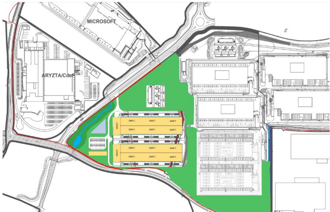
Figure 2.3 Double storey data centres & Admin office option
